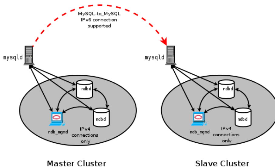
Figure 21.46 Replication Between SQL Nodes Connected Using IPv6
