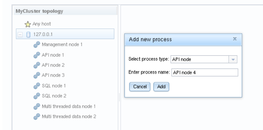
Figure 21.10 NDB Cluster Auto-Installer Add Process Dialog
