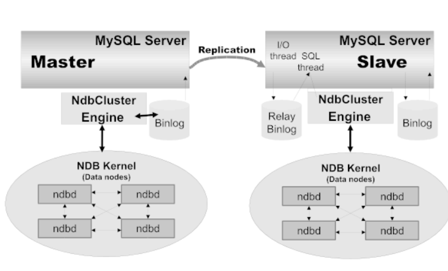
Figure 21.43 NDB Cluster-to-Cluster Replication Layout
