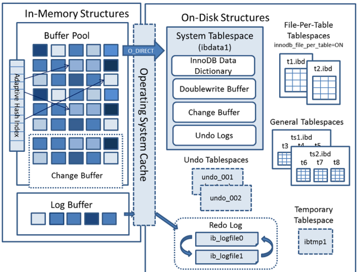
Figure 14.1 InnoDB Architecture
