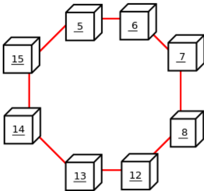
Figure 21.39 Circular Arrangement of NDB Cluster Nodes
