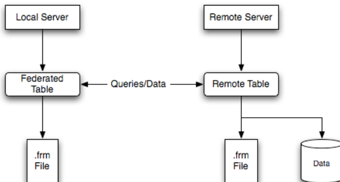
Figure 15.2 FEDERATED Table Structure
